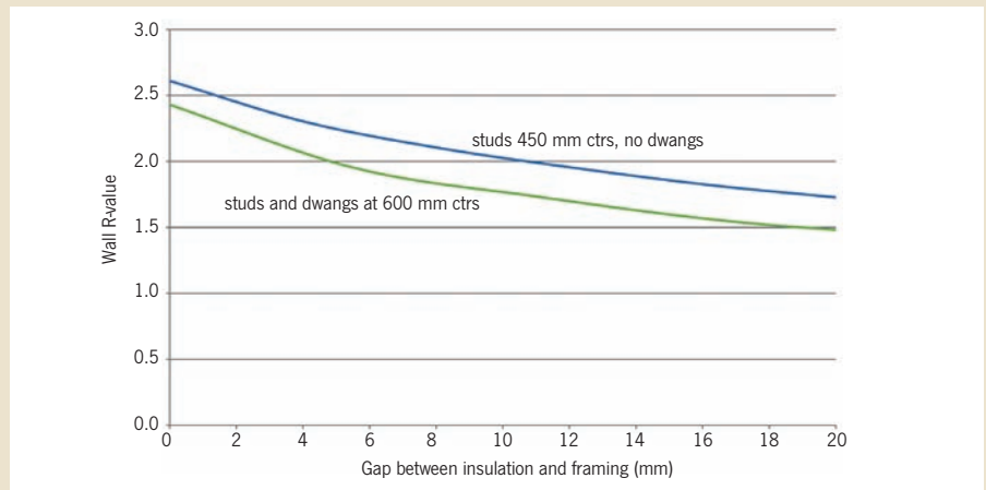
Figure 2: The impact of edge gaps on the system R-value.
