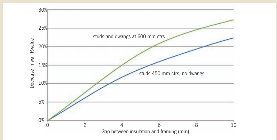
Figure 3: Modelling results for small gaps.
