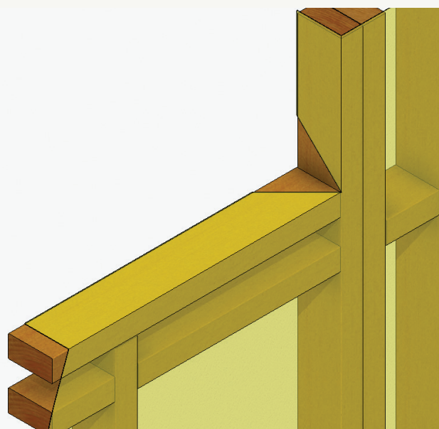
Step 1 Construction sequence.
